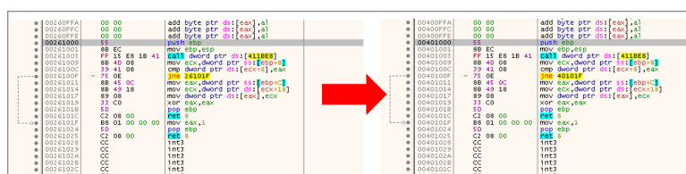
Figure 53 – Copying of the loader from 0x00260000 to 0x00400000
