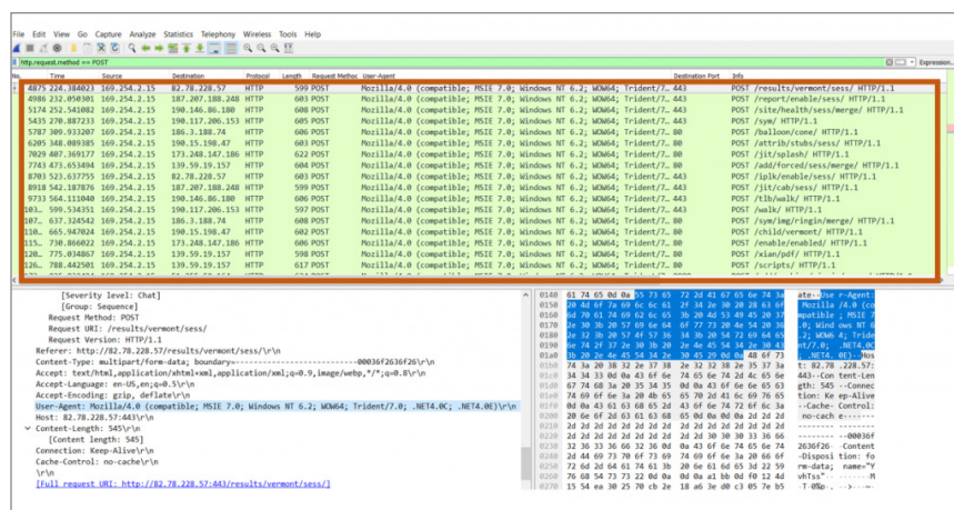
Figure 20 – HTTP POST requests to C2 servers
