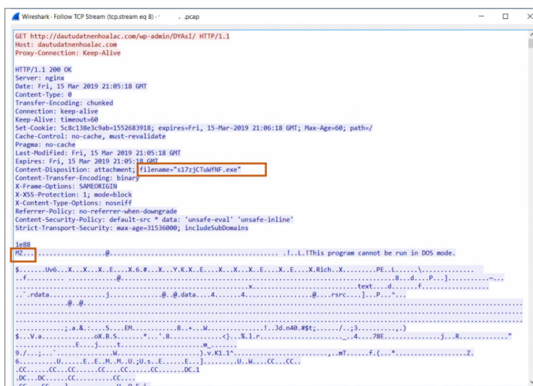
Figure 16 – HTTP GET request that downloads the Emotet loader
