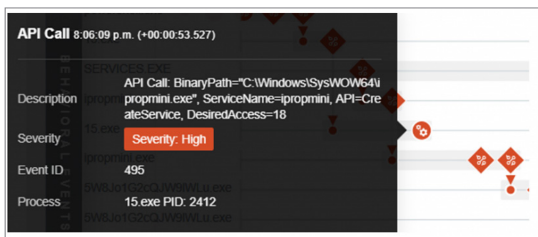
Figure 18 – Service creation to establish persistence
