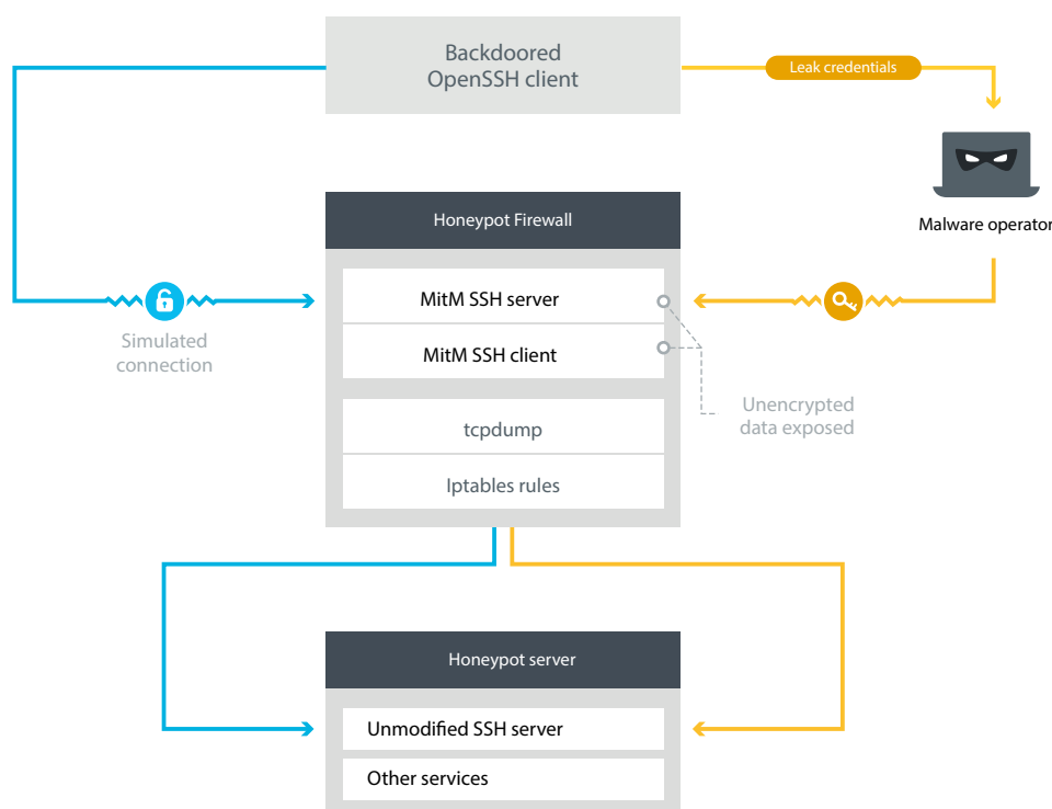
Figure 7 // Honeypot infrastructure
